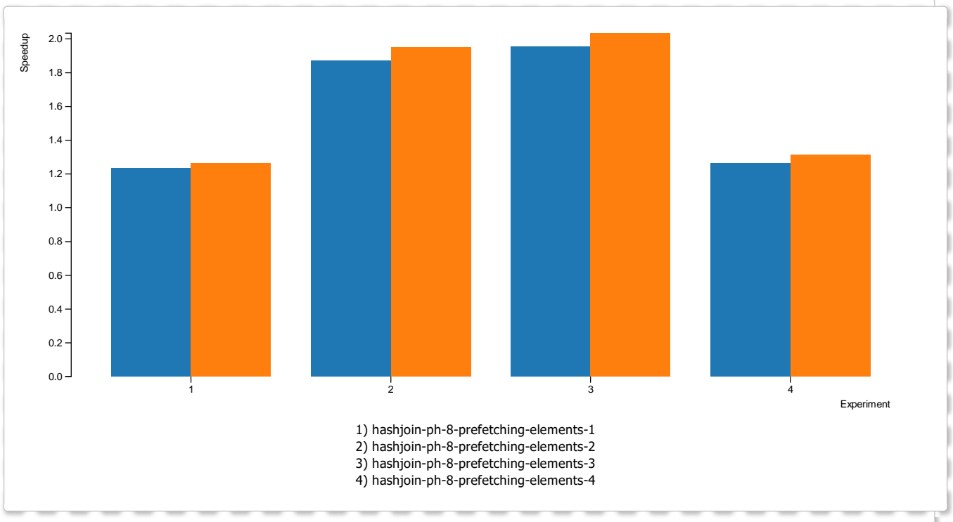
Figure 7 (hashjoin-ph-8)
