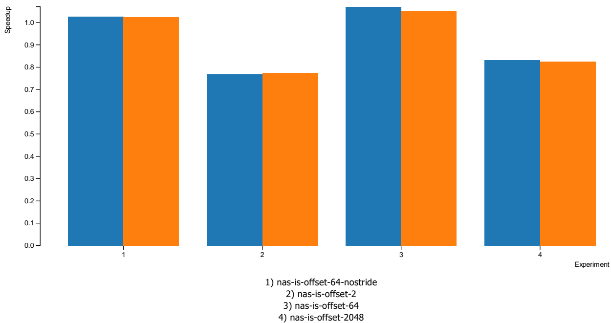
Figure 4 (graph500-s16)
