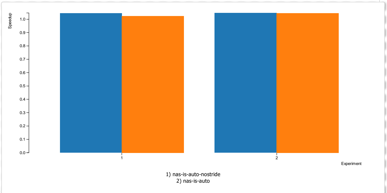
Figure 5 (randacc)
