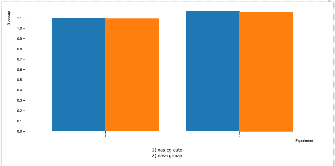
Figure 4 (nas-is)
