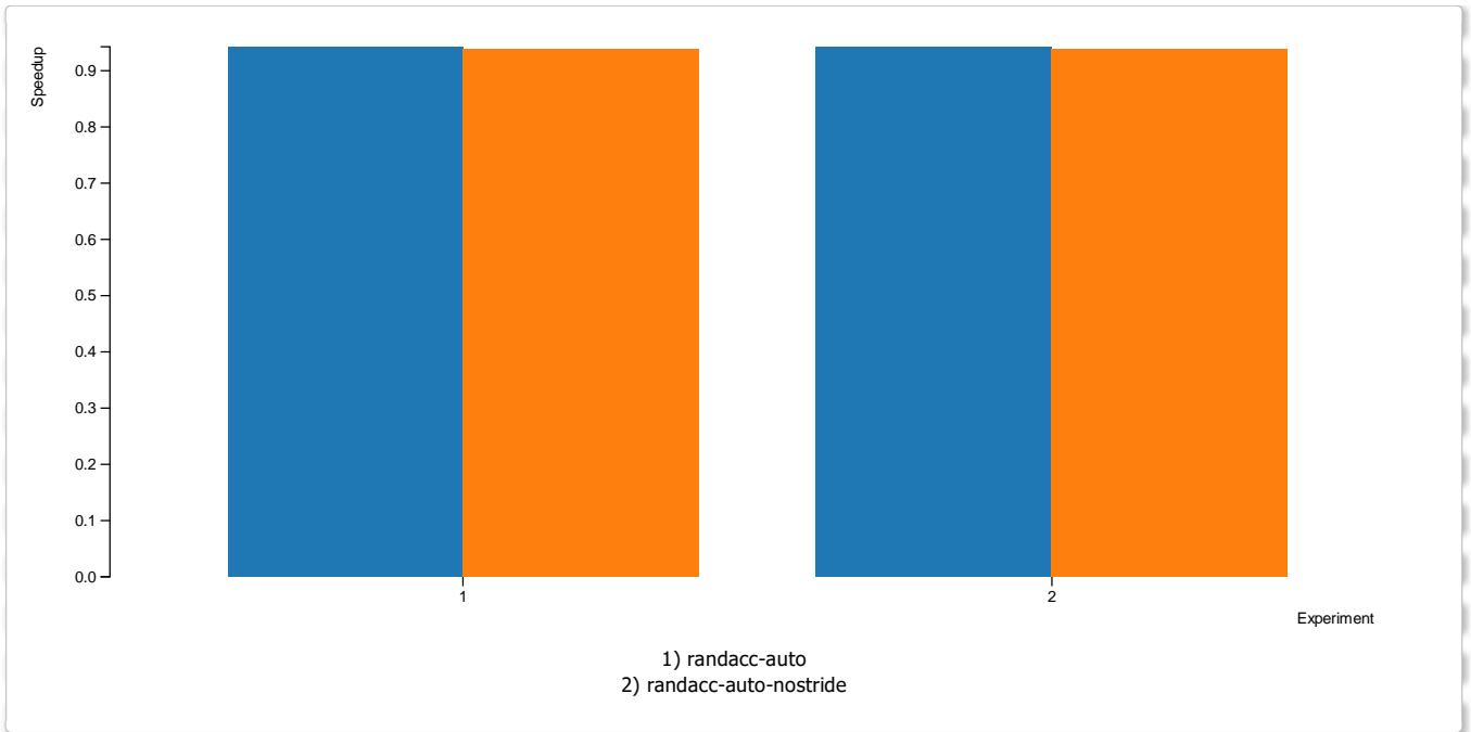
Figure 6 (hashjoin-ph-2)
