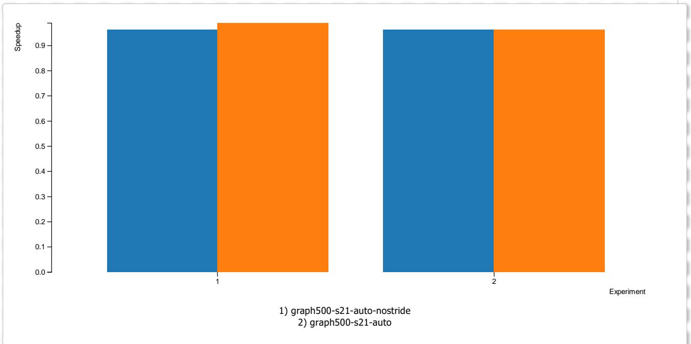
Figure 5 (hashjoin-ph-2)
