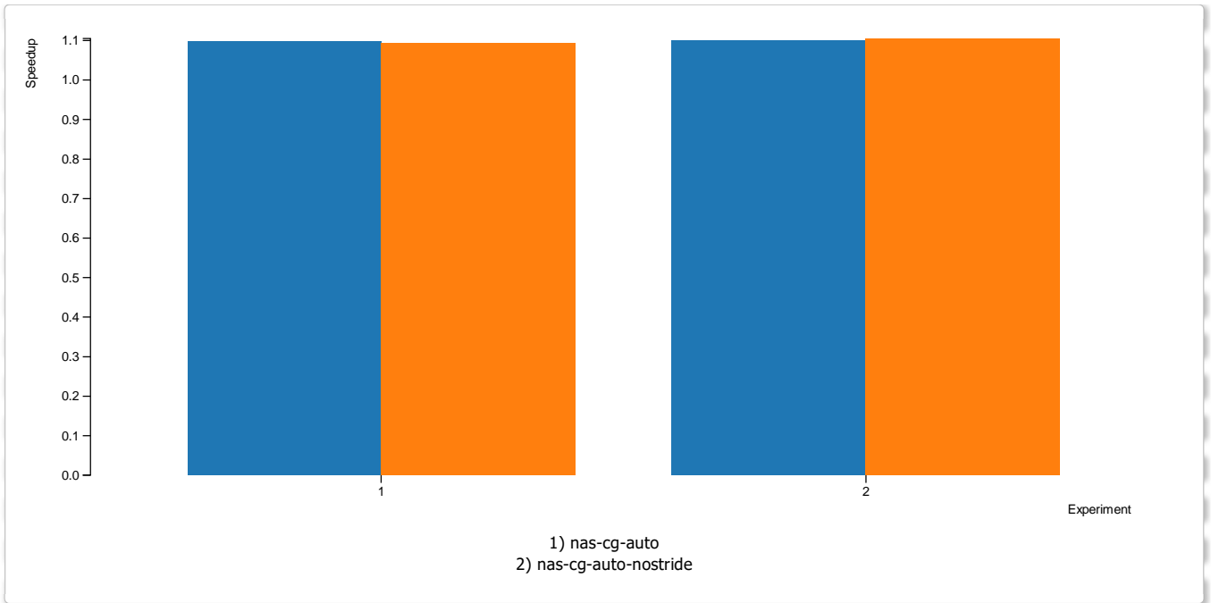
Figure 5 (nas-is)
