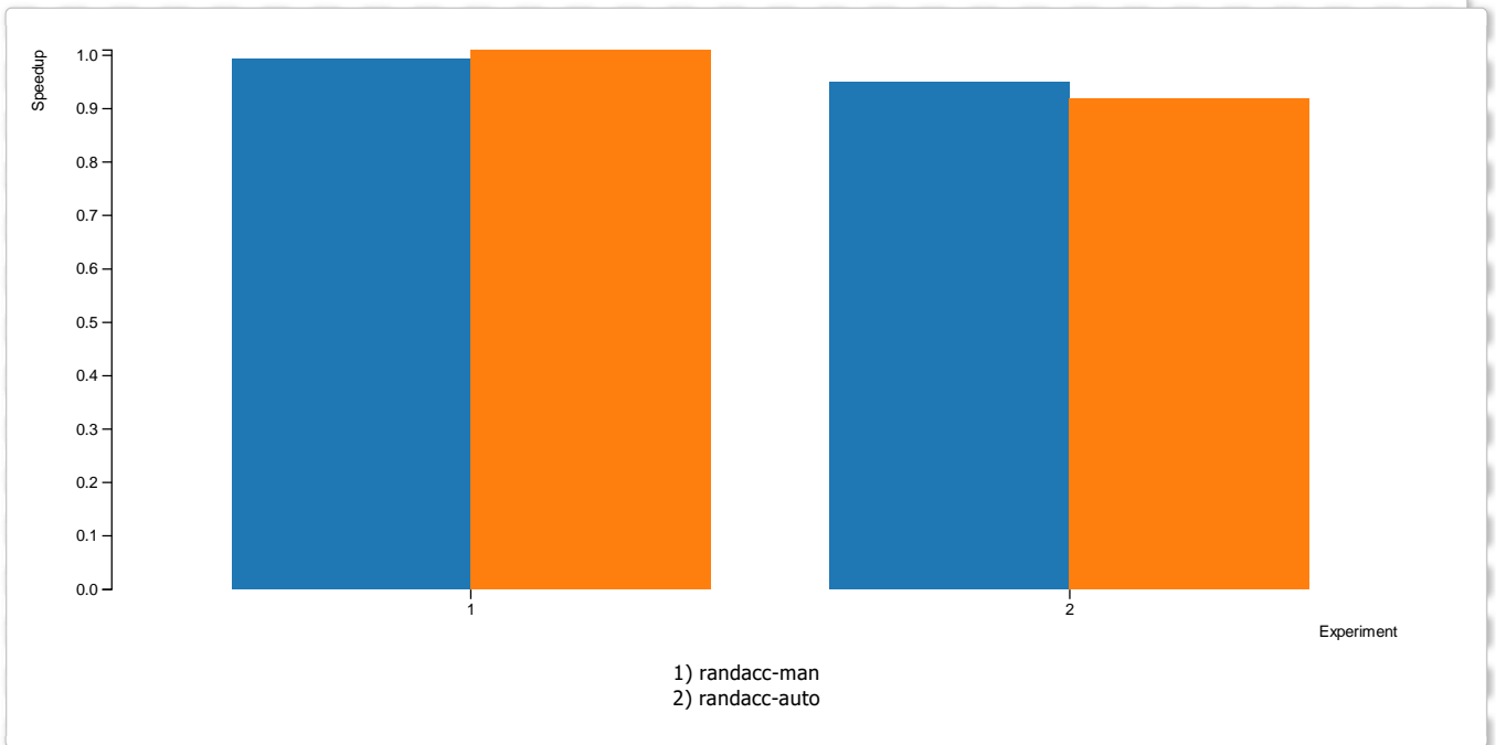
Figure 5 (graph500-s16)
