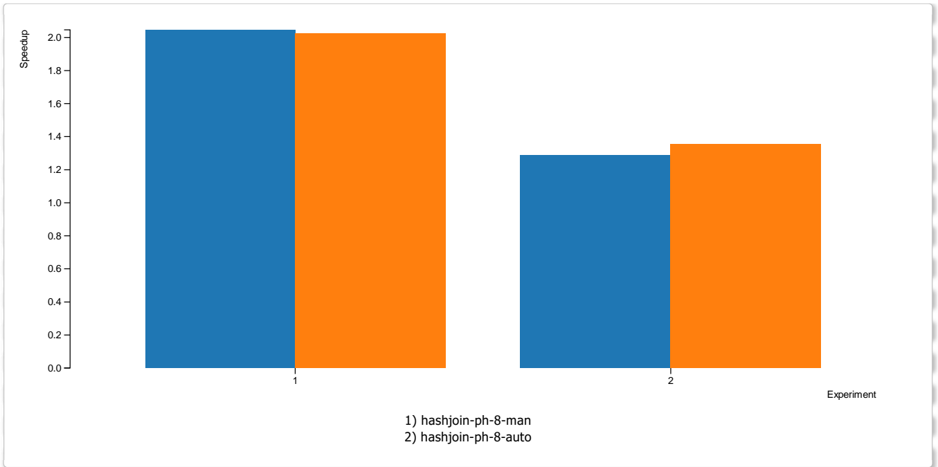
Figure 4 (nas-cg)
