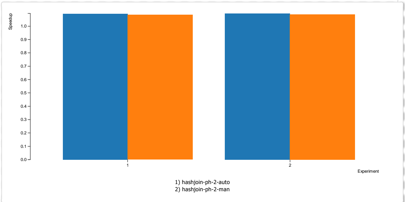
Figure 4 (hashjoin-ph-8)
