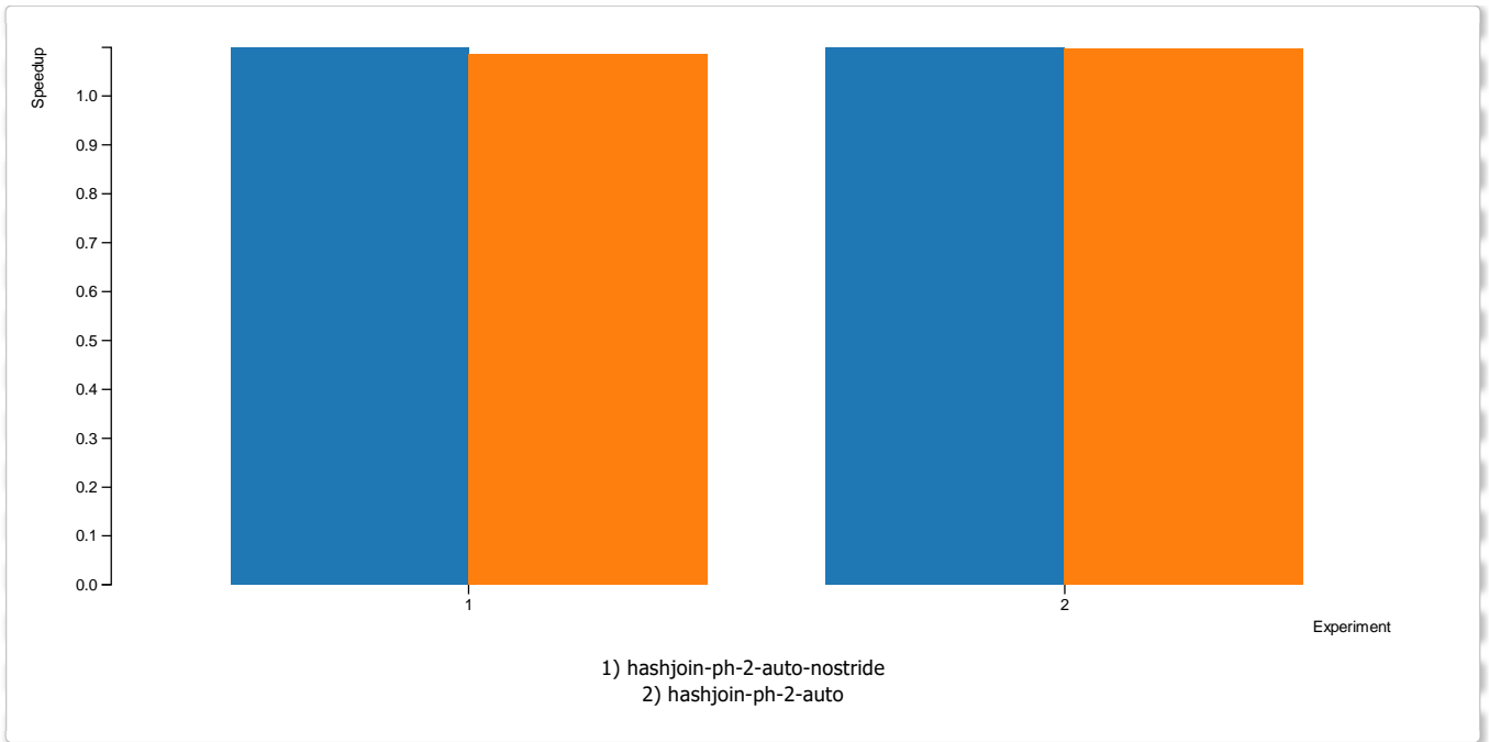
Figure 5 (hashjoin-ph-8)
