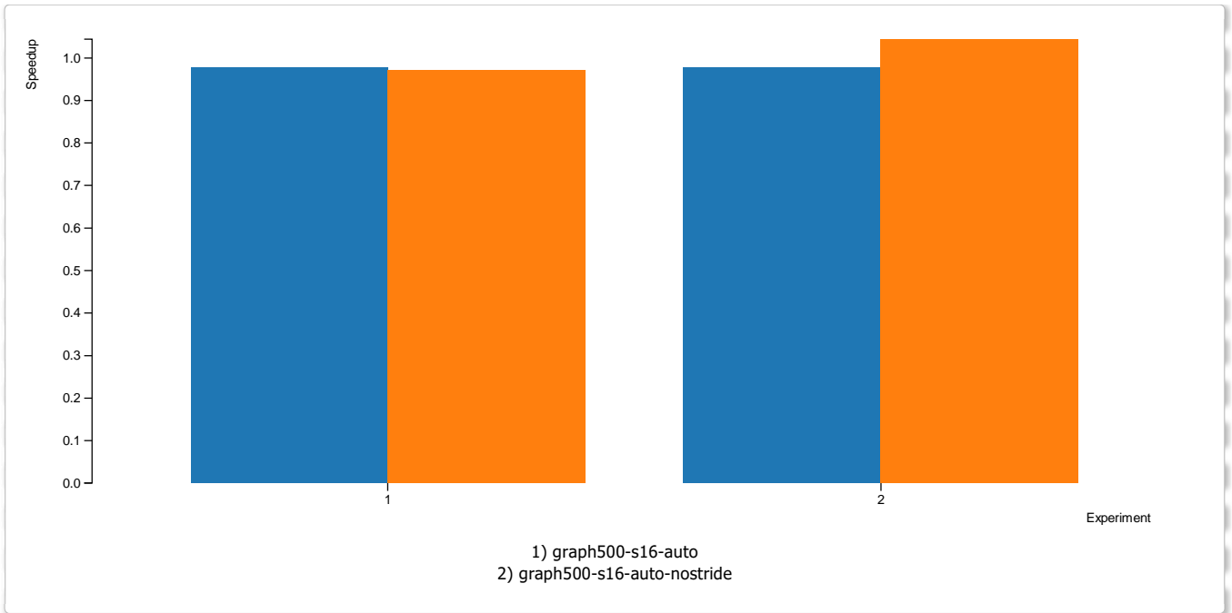
Figure 5 (graph500-s21)
