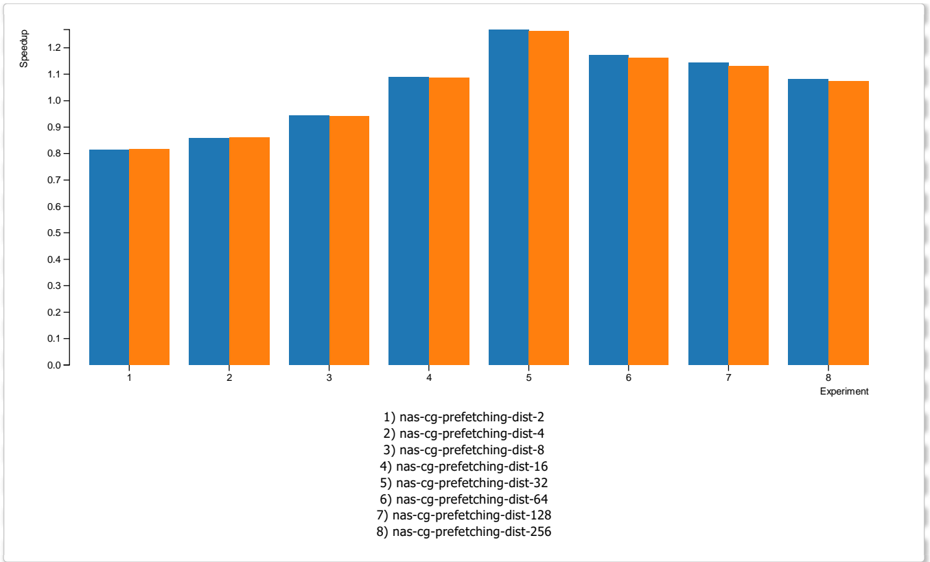
Figure 6 (nas-is)
