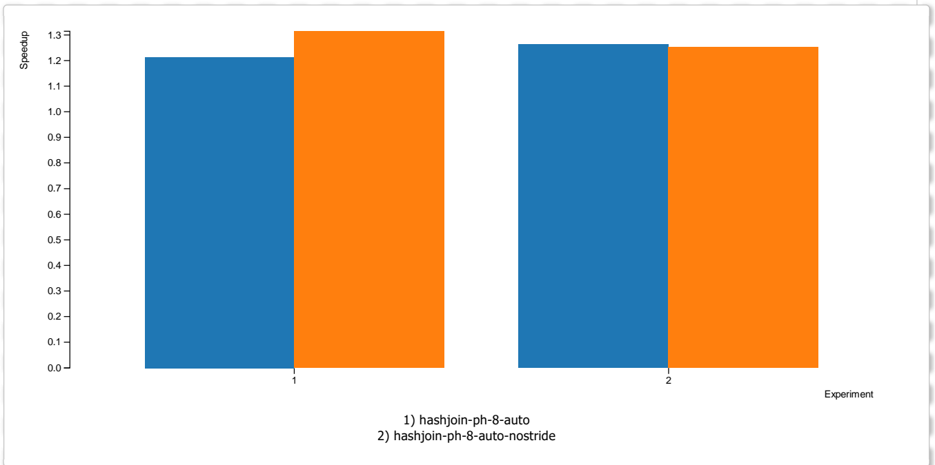
Figure 5 (nas-cg)
