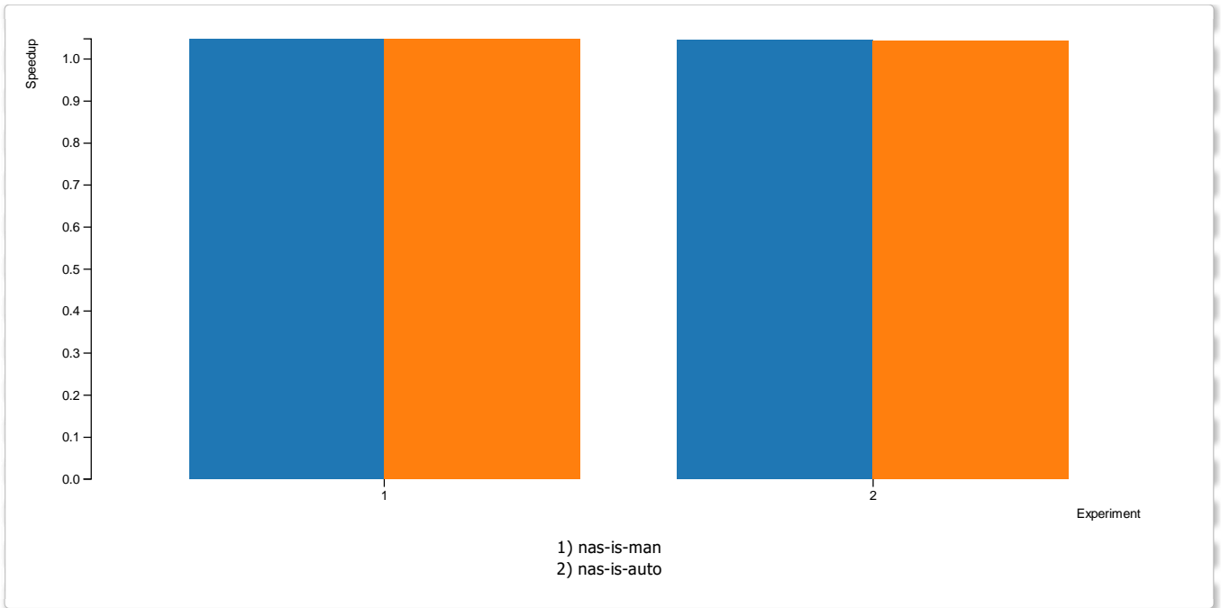
Figure 4 (randacc)
